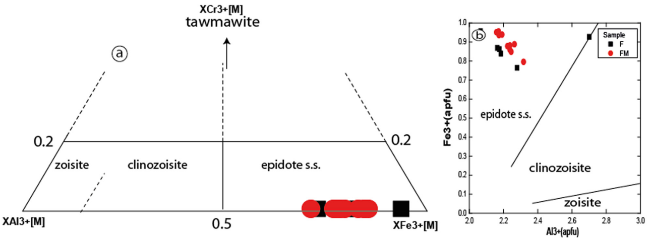
Figure 17: (a) Classification of minerals in the epidote group of the studied area on a triangular diagram based on [30]. ( XFe^{3+} = Fe^{3+} / (Fe^{3+} + Al^{3+} - 2 + Cr^{3+}) , XCr^{3+} = Cr^{3+} / (Fe^{3+} + Al^{3+} - 2 + Cr^{3+}) , XAl^{3+} = (Al^{3+} - 2) / (Fe^{3+} + Al^{3+} - 2 + Cr^{3+}) ). (b) Fe^{3+} vs Al^{3+} .
