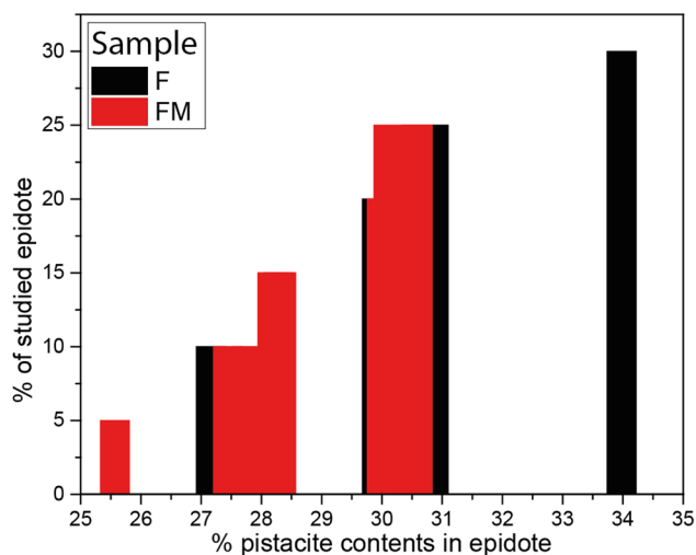
Figure 18: Percentage of pistacite in the epidote of the study area, derived from alteration of plagioclase (F) and ferromagnesian (FM) minerals.
