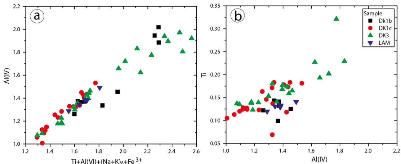
Figure 12: (a) Almost perfect linear variation of Al^{IV} with Al^{VI} + Fe^{3+} + Ti + (Na + K) [21]. (b) Ti diagrams relative to Al^{IV} in amphiboles. All amphiboles have less than 0.5 Ti atom in the structural formula.
