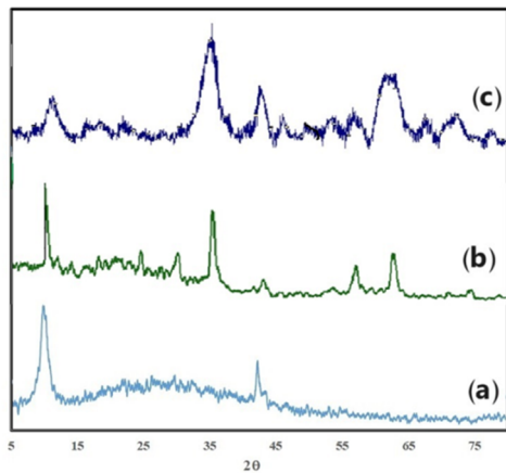
Fig. 2. XRD patterns of a) GO, b) MGO and c) MGO-IDA
