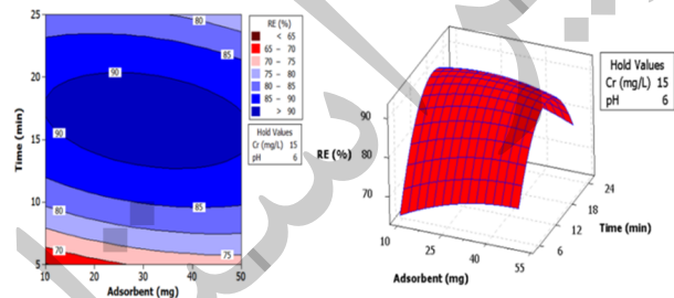
Fig. 6. Two and three-dimensional diagrams of the effect of adsorption time and adsorbent weight on absorption efficiency
