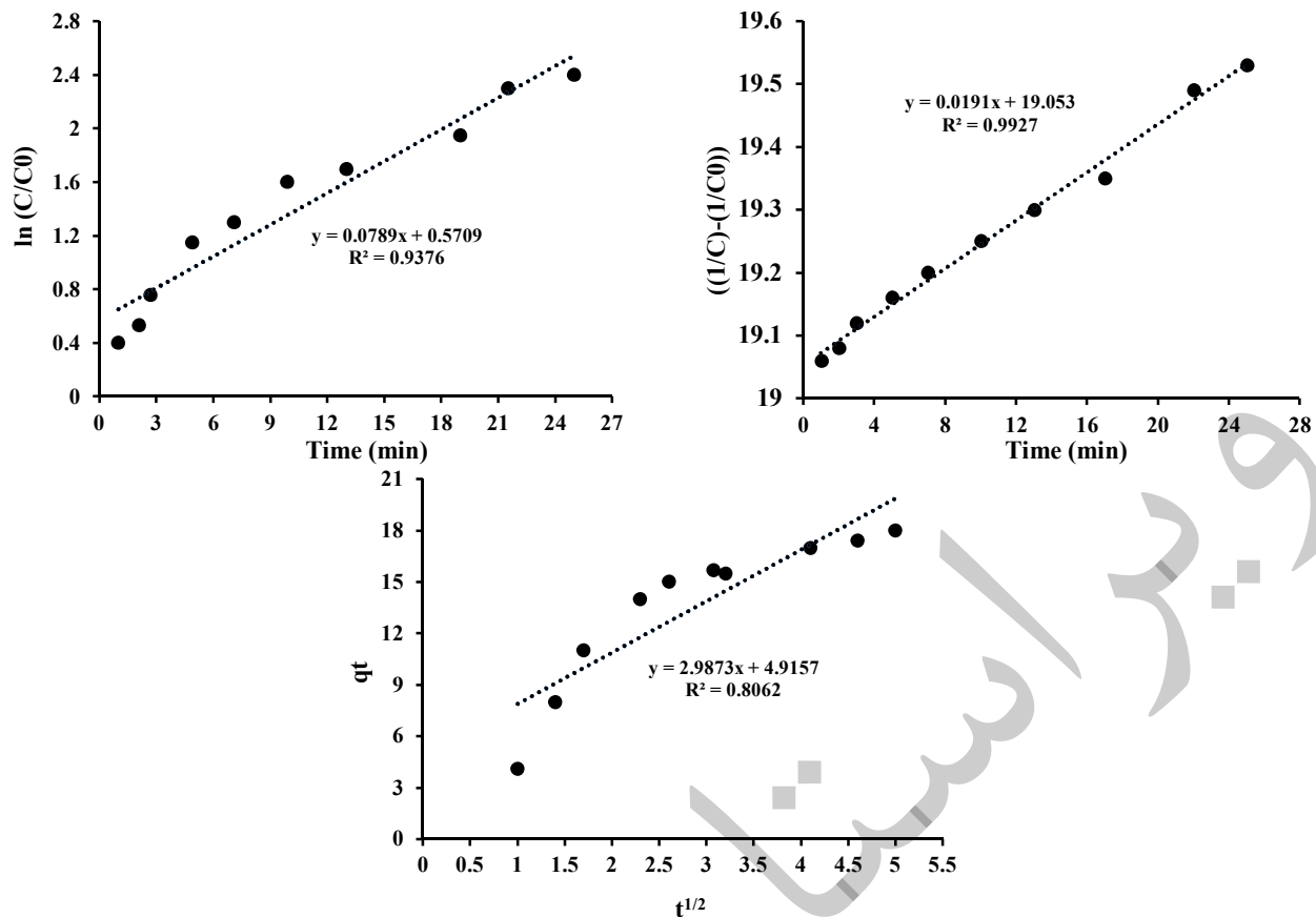
Fig. 9. Fit of a) pseudo first, b) second order and c) intra-particle diffusion kinetic models for the adsorption of \text{Cr}^{3+} onto the MGO-IDA
