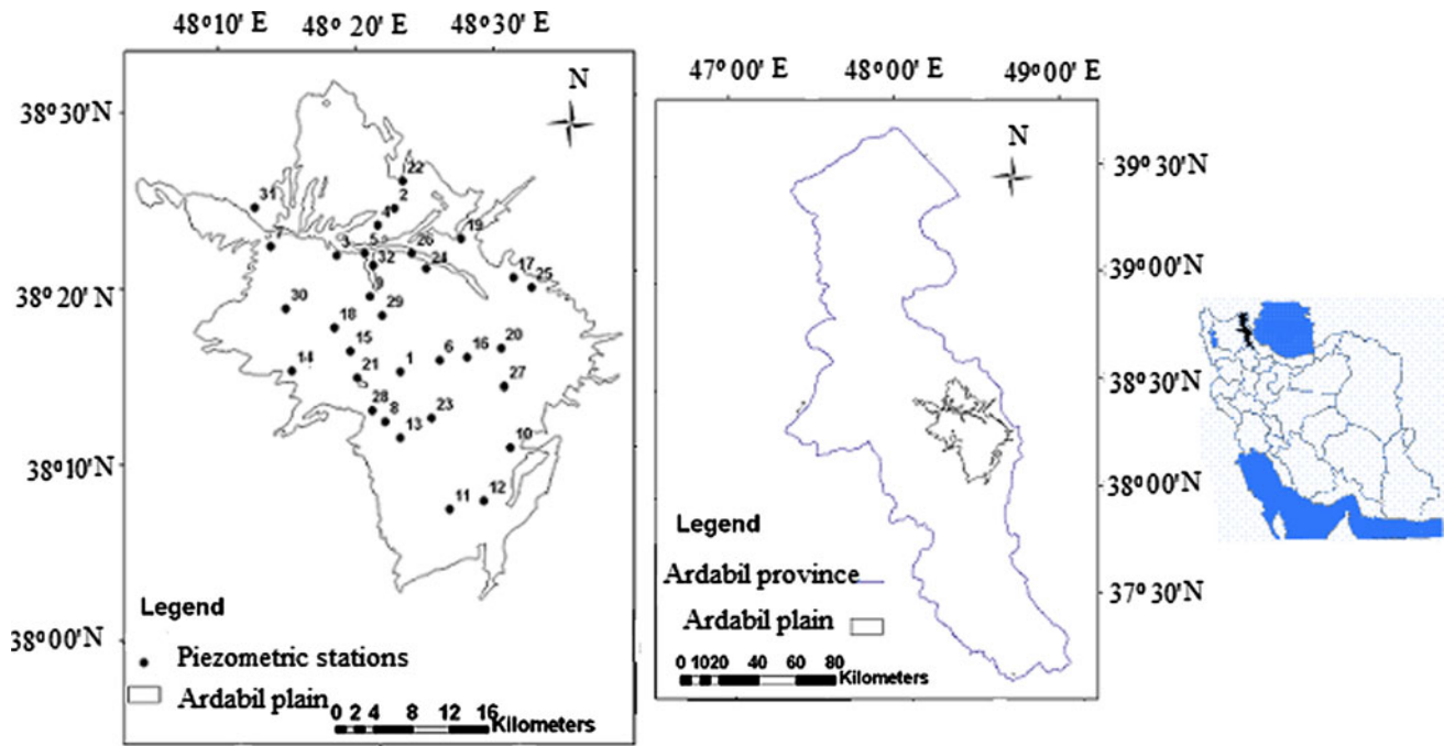
Fig. 1 Study area map, Ardabil plain, Iran
