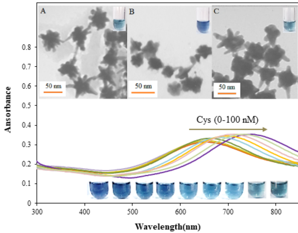
A colorimetric sensor for cysteine based on the gold nanostars
